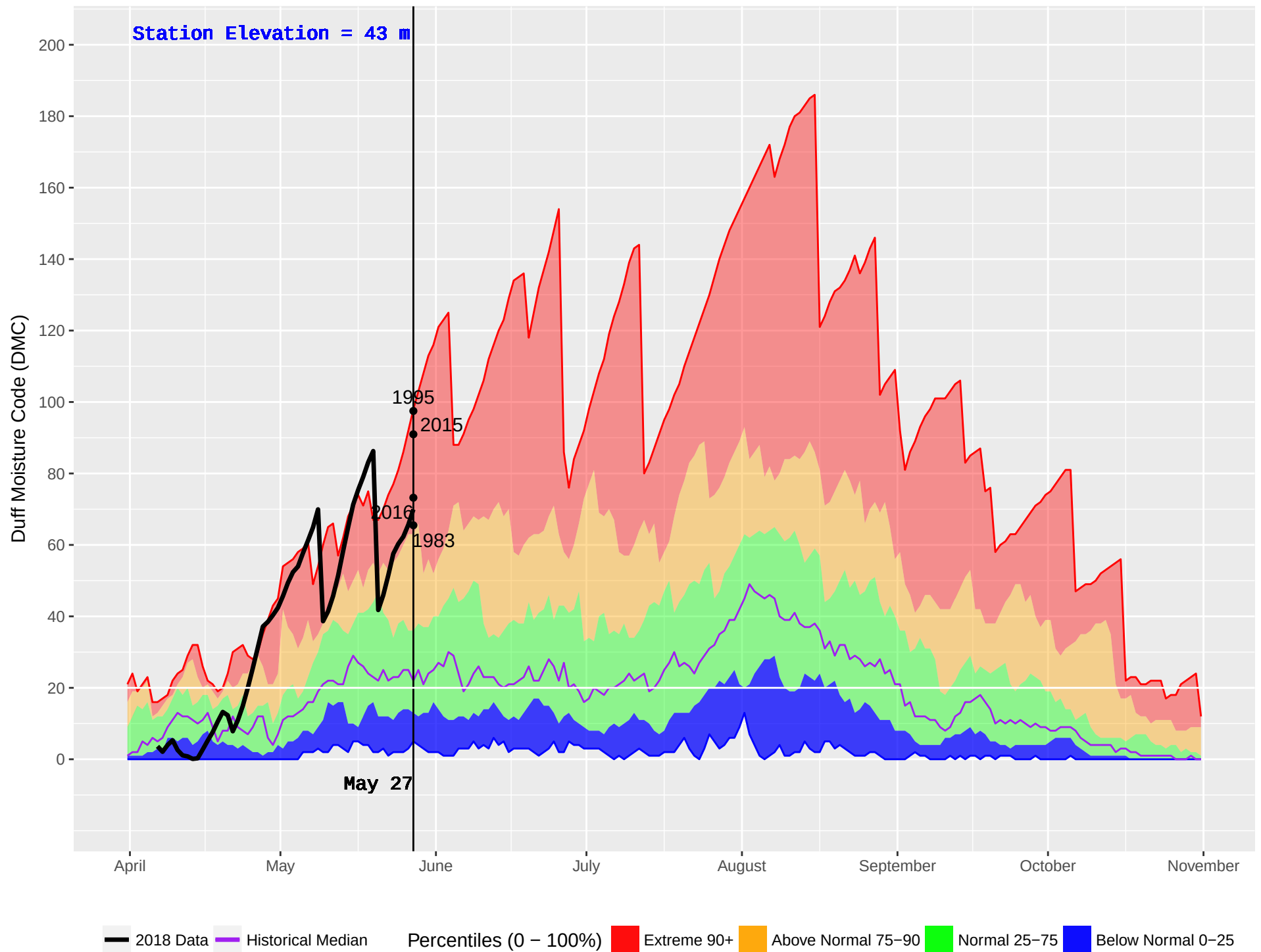
TOBA CAMP (75) : Historical (1970–2016) and Current (2018) Noon Duff Moisture Code (DMC)
