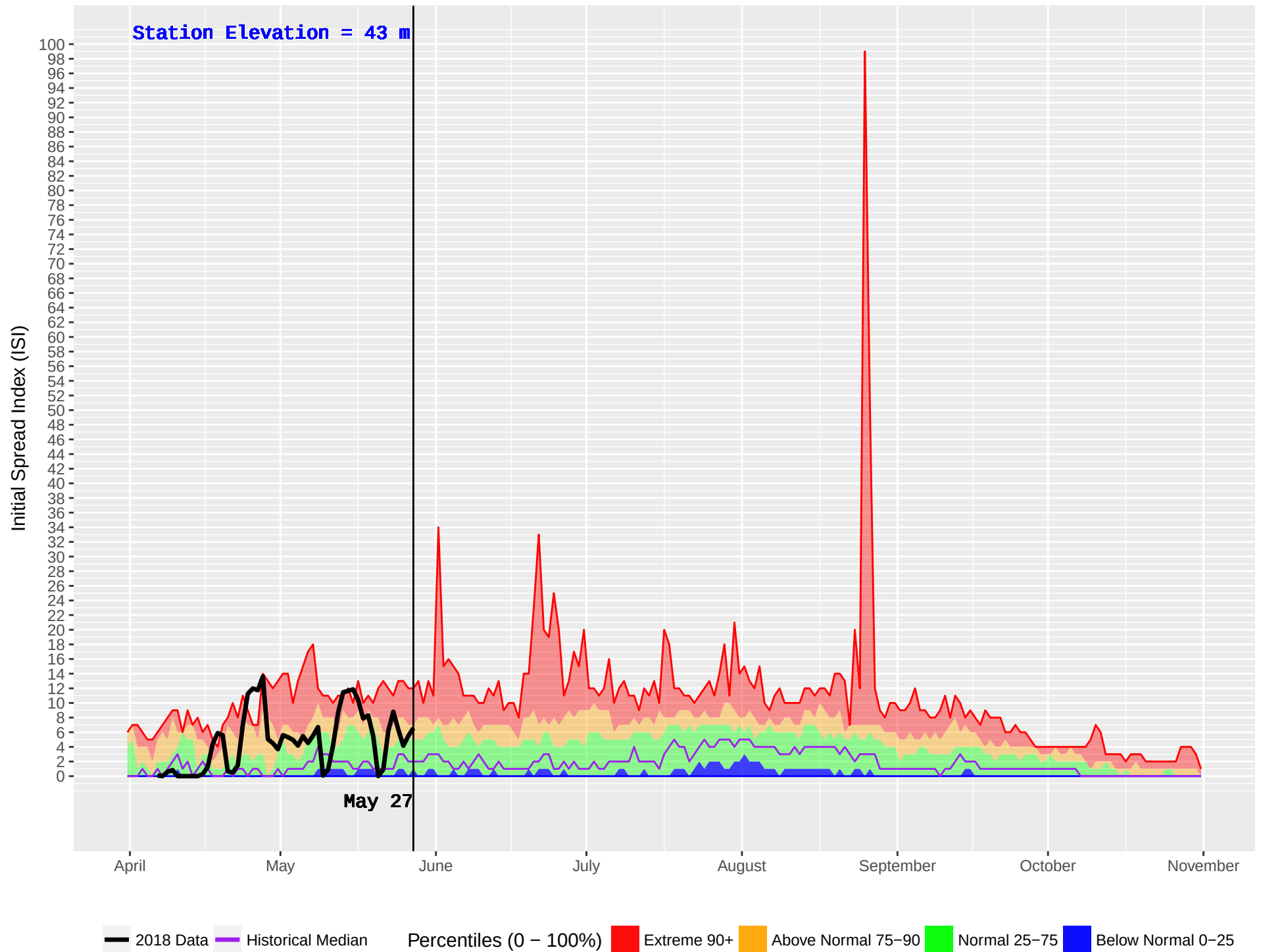
TOBA CAMP (75) : Historical (1970–2016) and Current (2018) Noon Initial Spread Index (ISI)
